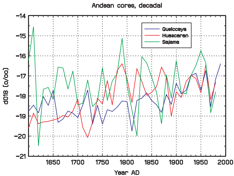
Figure 4. Andean d^{18}\text{O} isotope ratio series, decadal averages constructed from 5-year averages in Thompson et al. [1] Data Set 2. Years indicate beginning of decade in question.
