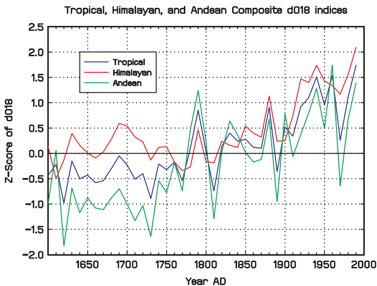
Figure 2. Composite d^{18}\text{O} Z-score index for 7 Himalayan and Andean ice cores, together with regional subindices, from Thompson et al. [1], Data Set 3, decadal averages. Years indicate beginning of decade in question.
