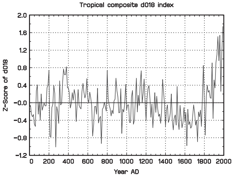
Figure 1. Composite d^{18}\text{O} Z-score for 7 Tibetan and Andean ice cores, decadal averages, from Thompson et al. [1], Data Set 3. Years indicate beginning of decade in question.
