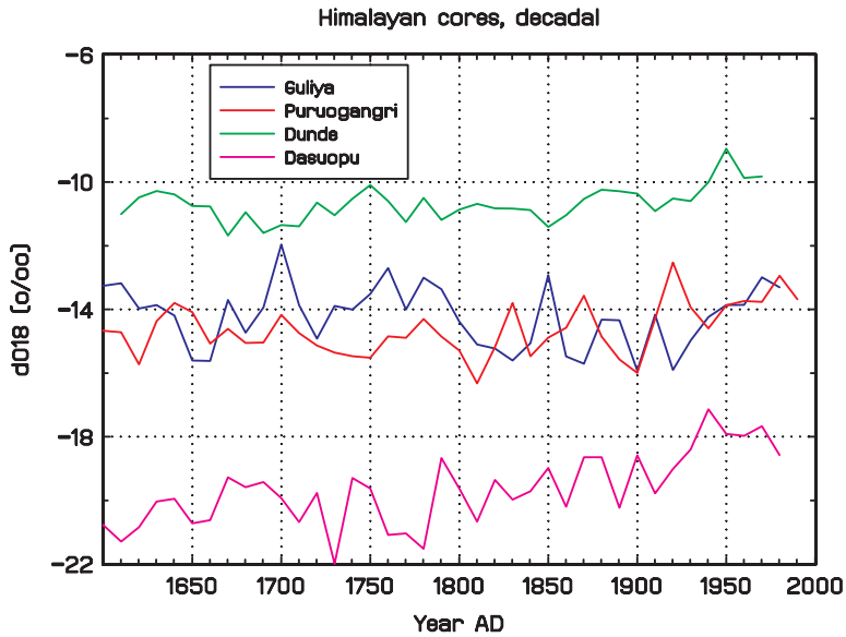
Figure 3. Himalayan d^{18}\text{O} isotope ratio series, decadal averages constructed from 5-year averages in Thompson et al. [1] Data Set 2. Years indicate beginning of decade in question.
